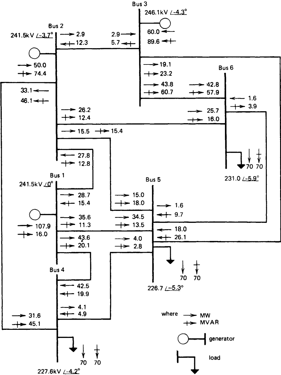
FIG. 4.8 Six-bus network base case AC power flow.
